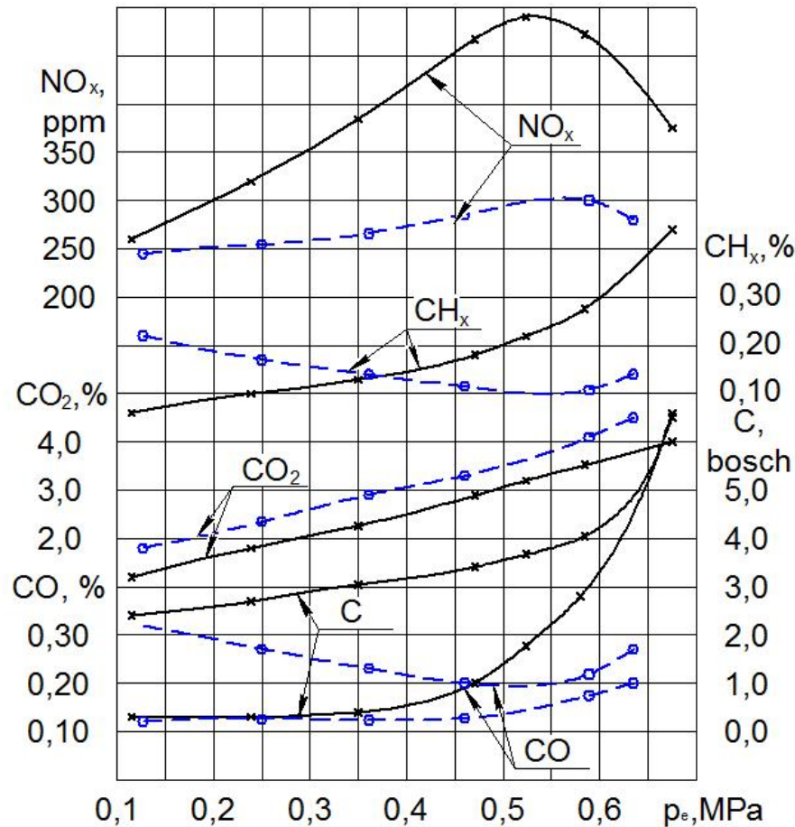
Figure 2b. The content of toxic components in the exhaust gases of a diesel engine 2H 10.5 / 12.0 when operating on diesel fuel and methanol with a separate supply depending on the load change with n = 1400 \text{ min}^{-1}
