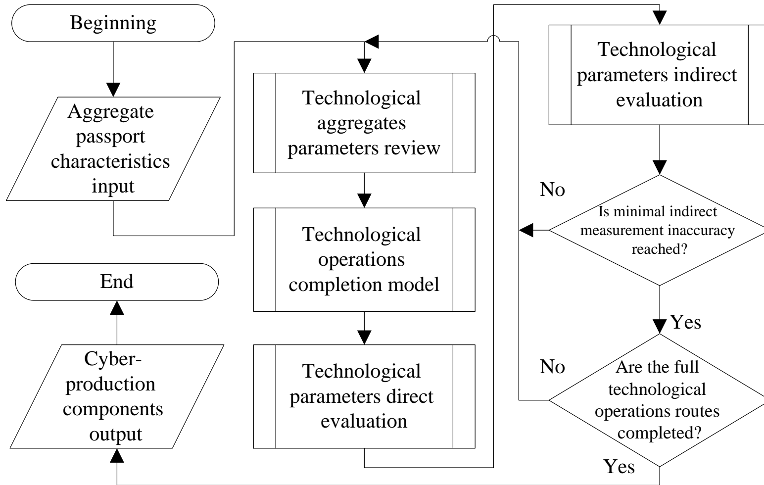
Figure 2. The cyber-production animation design algorithm in a multi-media environment.
