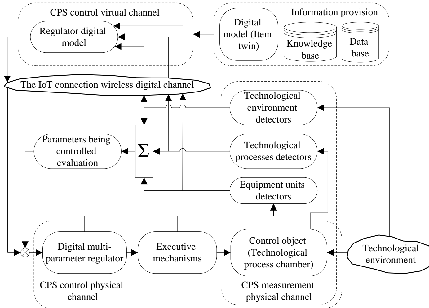
Figure 1. The CPP information environment (with one CPS unit control example).
